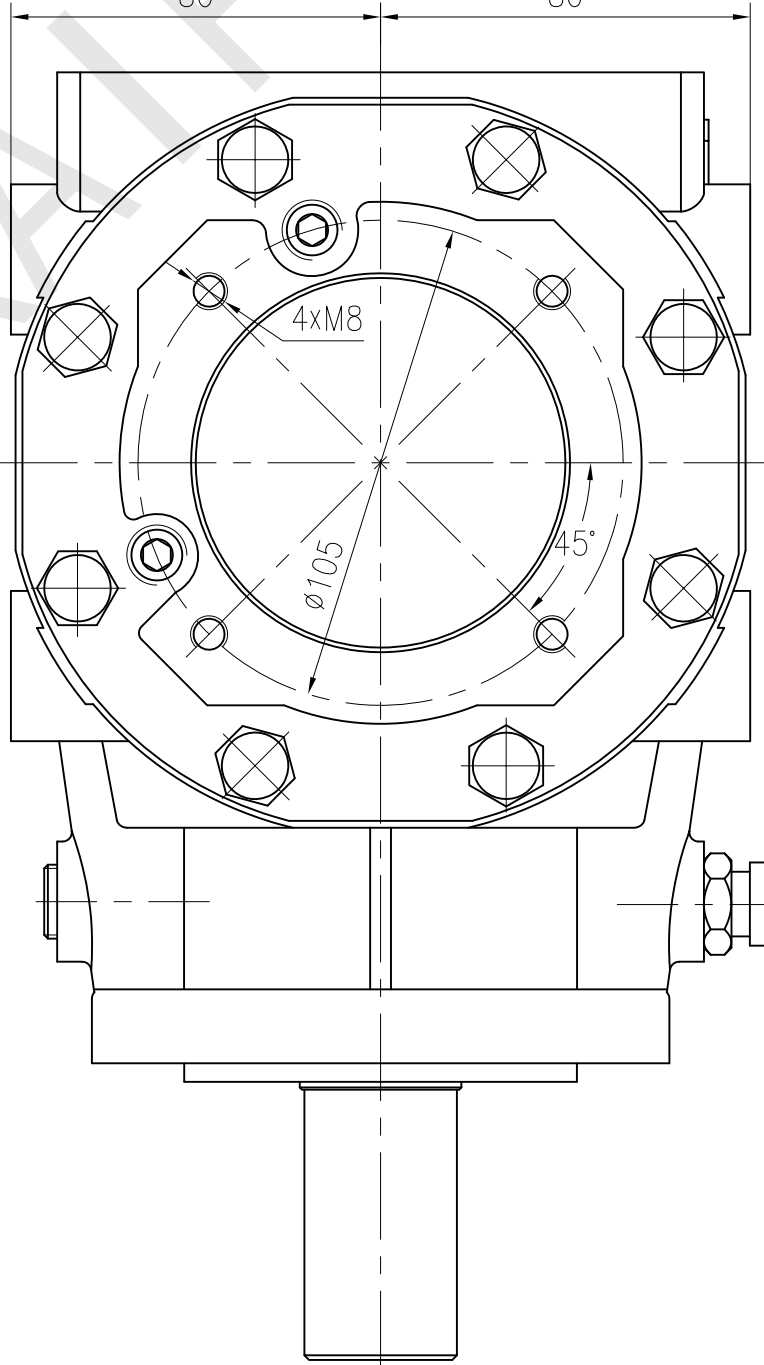
KF030R300Z0300 View from D
