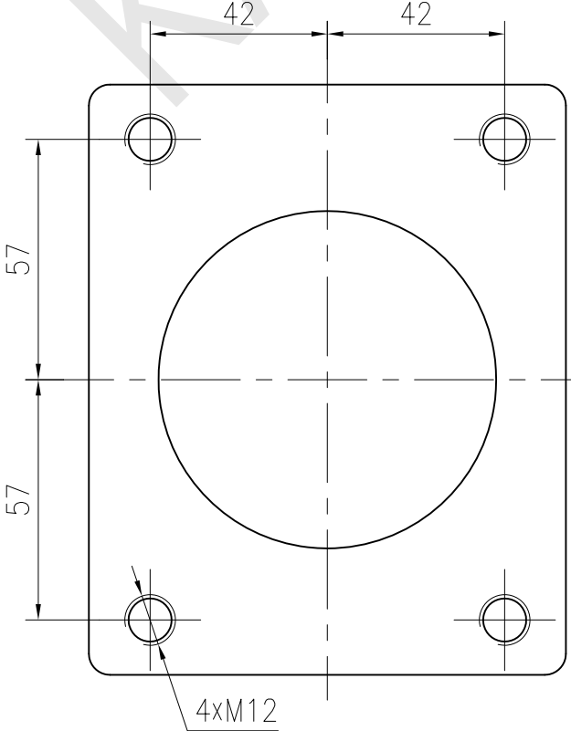
View from C
