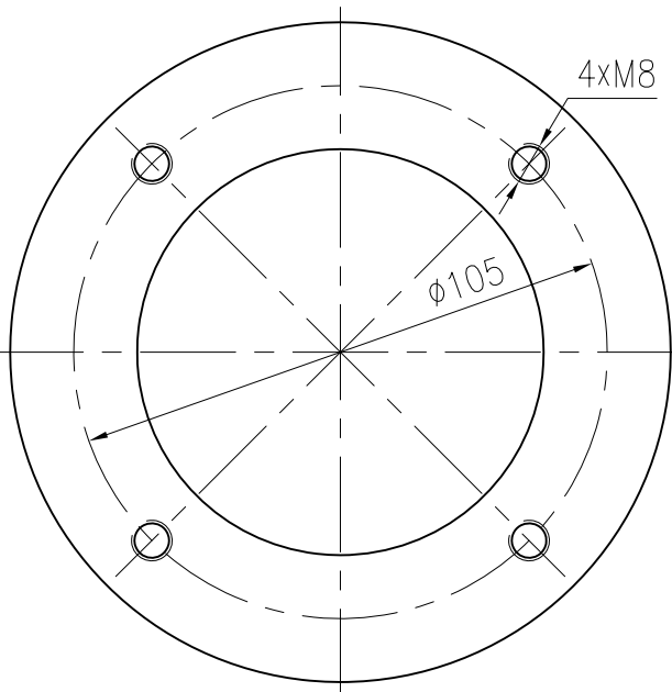
KF030R300Z0200 View from A
