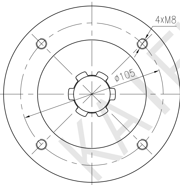
KF030R300Z0100/0300 View from A
