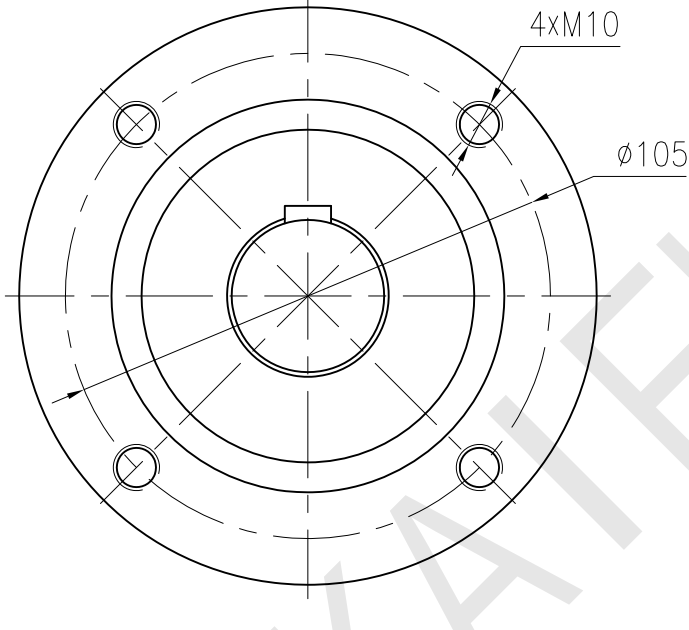
View from B
