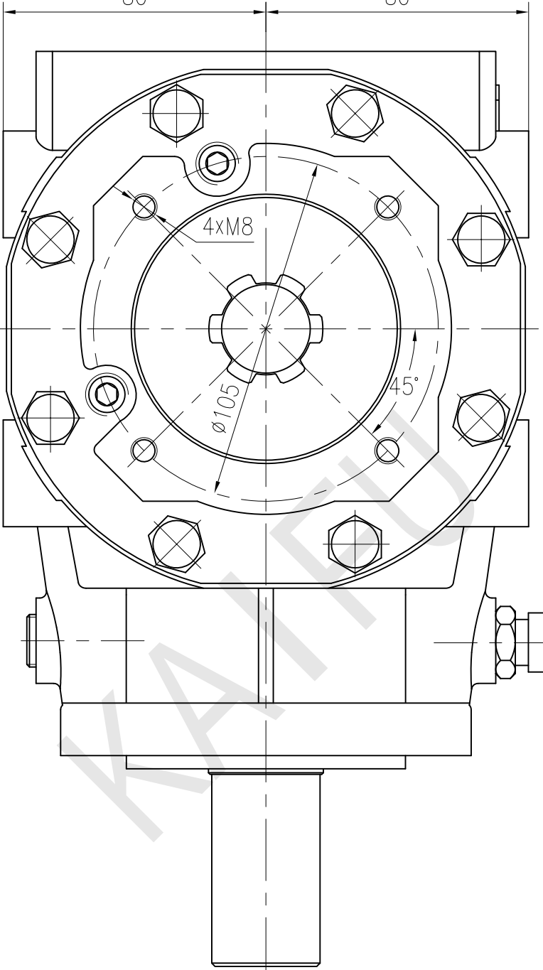
KF030R300Z0100/0200 View from D
